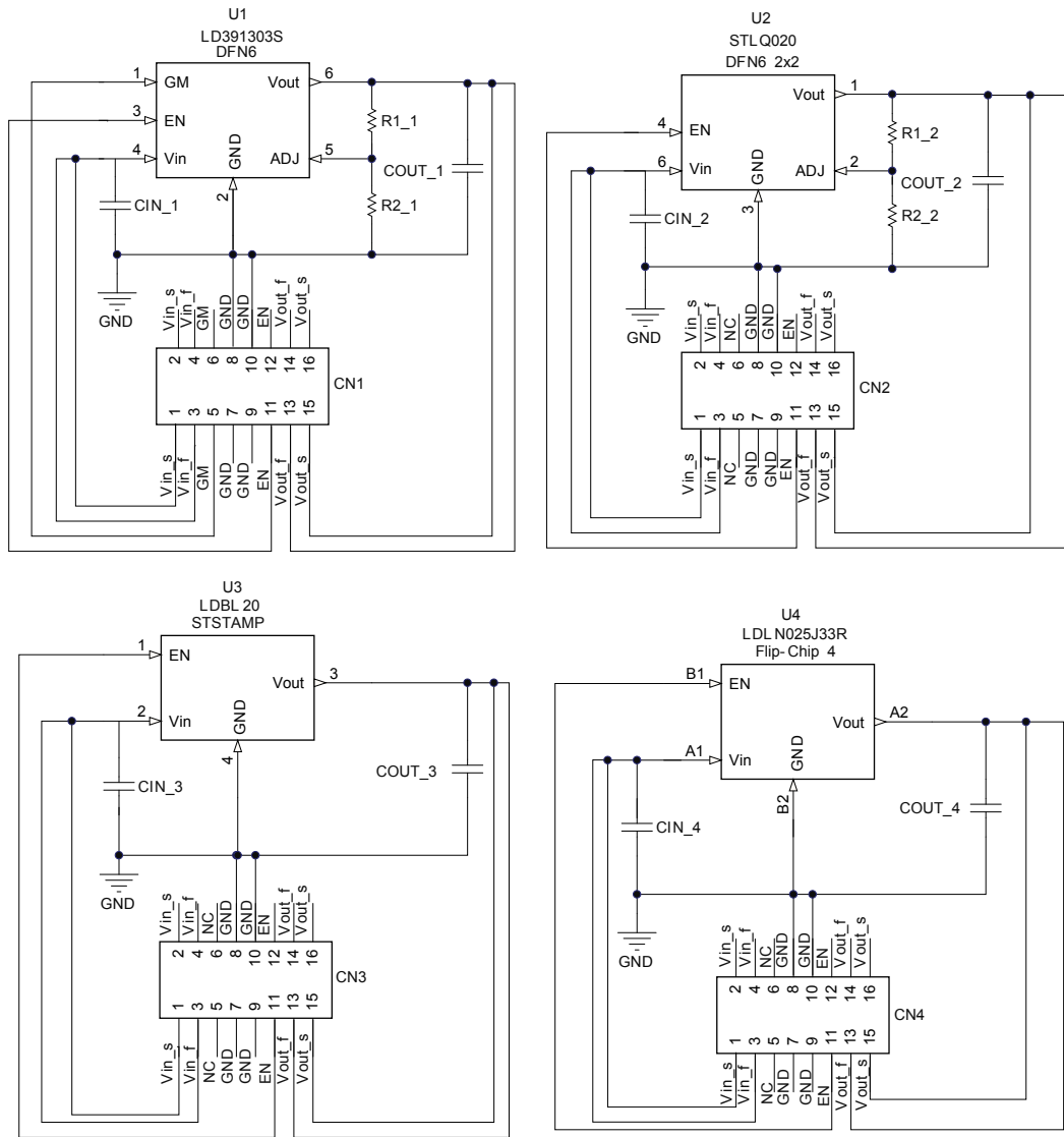
Figure 1: STEVAL-LDO001V1 circuit schematic
