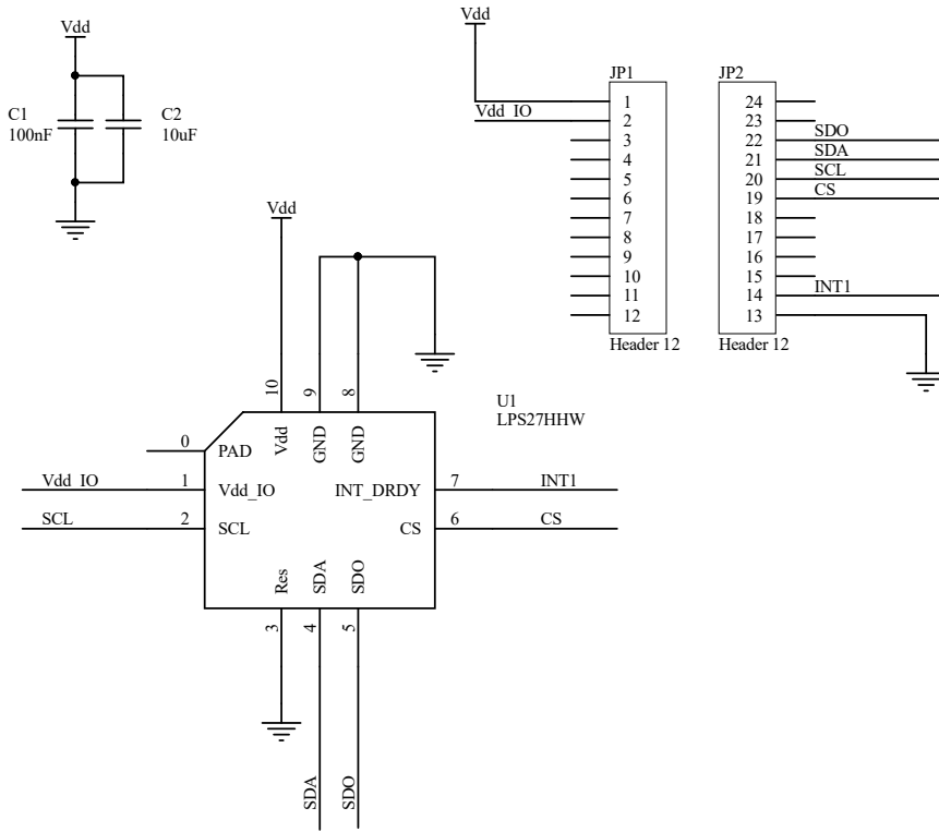
Figure 1: STEVAL-MKI213V1 board schematic
