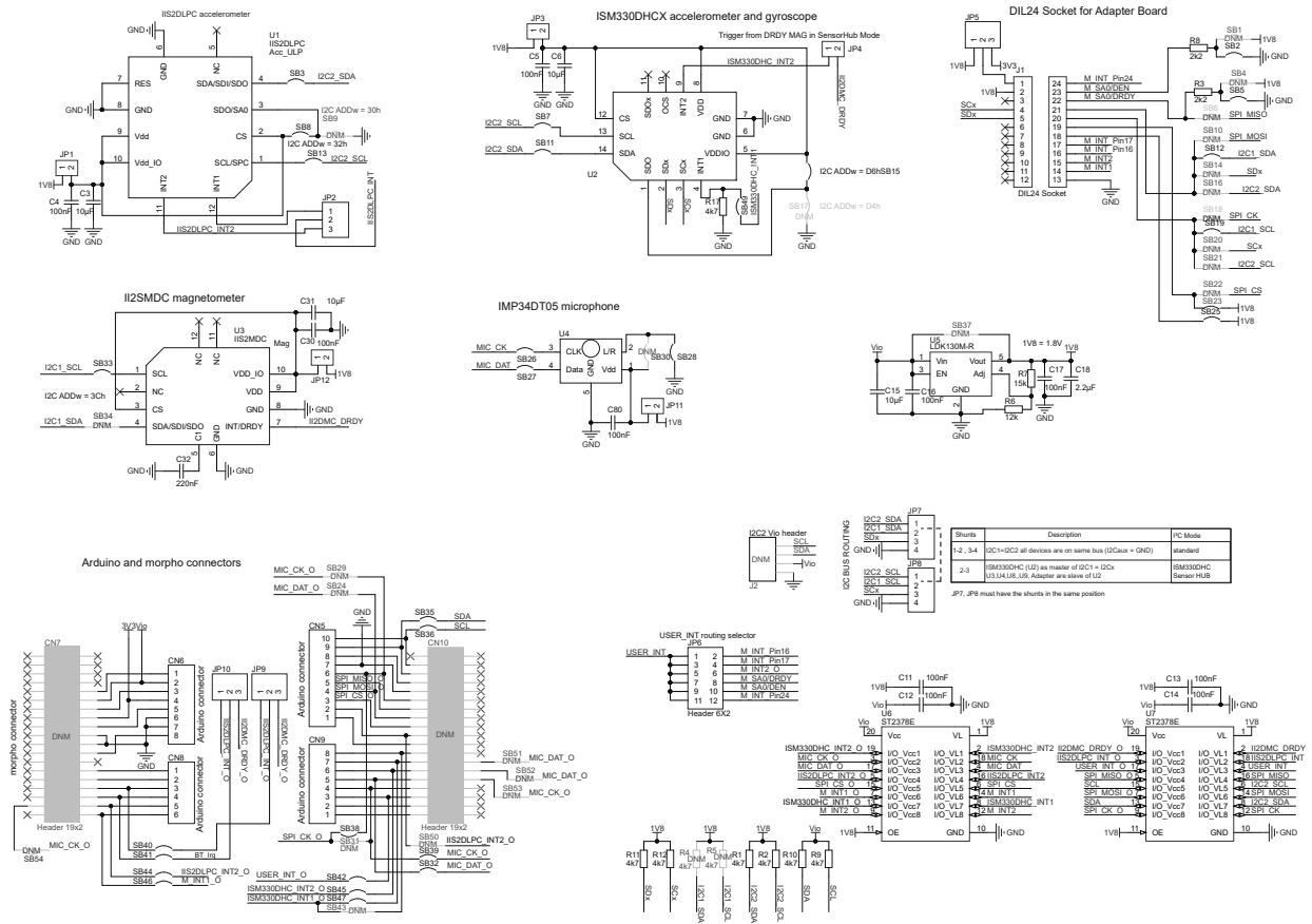
Figure 1: X-NUCLEO-IKS02A1 circuit schematic
