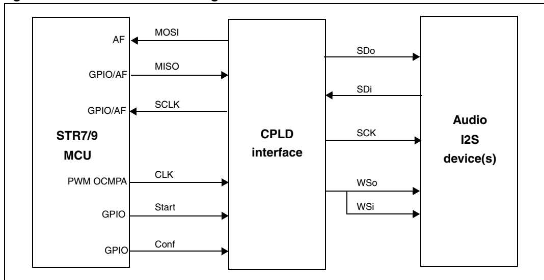
Figure 4. SPI to I2S CPLD bridge connections
