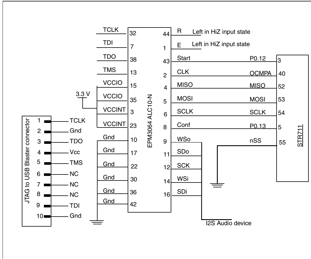
Figure 7. MAX3000A and STR711 SPI connections
