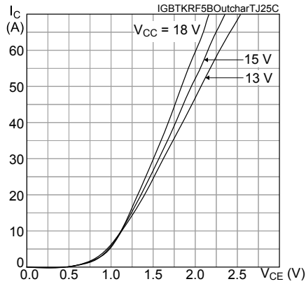
Figure 9. Output characteristics
