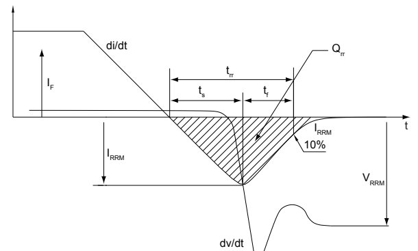
Figure 30. Diode reverse recovery waveform
