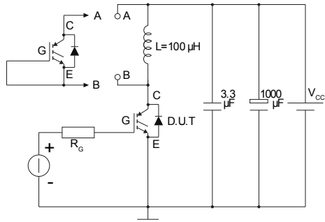
Figure 27. Test circuit for inductive load switching
