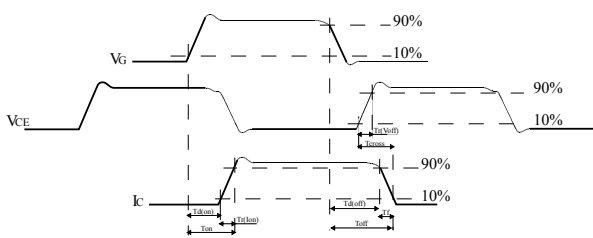
Figure 29. Switching waveform
