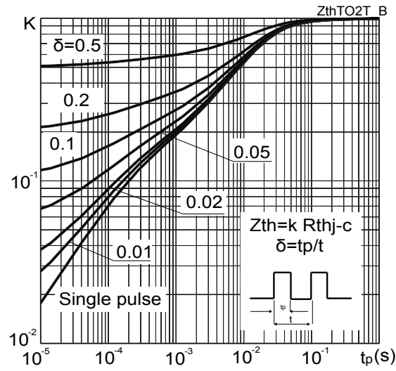
Figure 25. Thermal impedance
